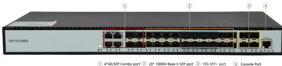
① 4*GE/SFP Combo port ② 20* 1000M Base-X SFP port ③ 10G SFP+ port ④ Console Port
